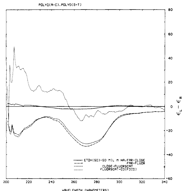
FIGURE 8: Scattering components for the different sectors of the scattering envelope for the DNA in Figures 6 and 7.
