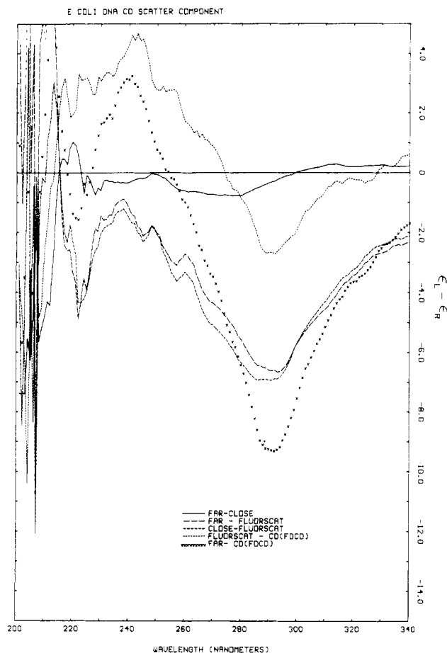
FIGURE 4: Difference CD curves giving the scattering components as a function of sectors in the scattering envelope. Note that the largest components are in the close minus flourescat sector, i.e., at right angles to the light beam.
