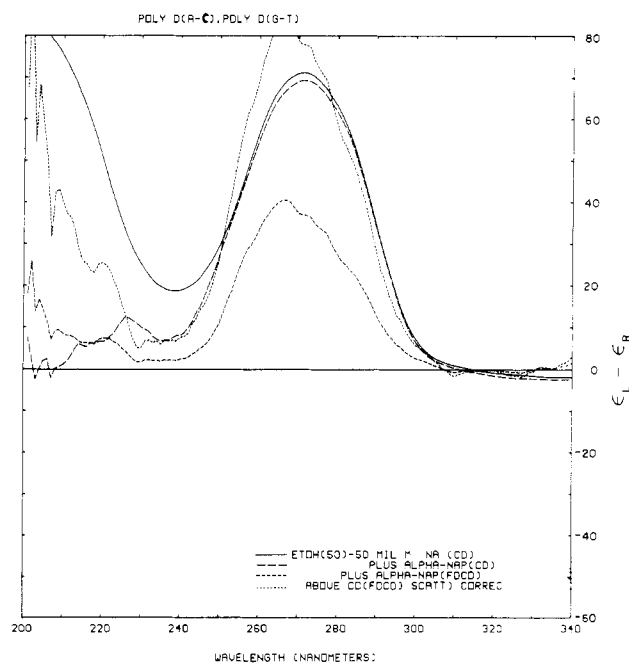
FIGURE 7: Correction by FDCD methods. The curve labeled plus alpha-NAP (CD) is the ordinary CD of the DNA plus the \alpha -NAP. The curve labeled plus alpha-NAP (FDCD) is the raw FDCD measurement, and the curve labeled CD(FDCD) scatt correc is the CD computed from the FDCD raw data.
