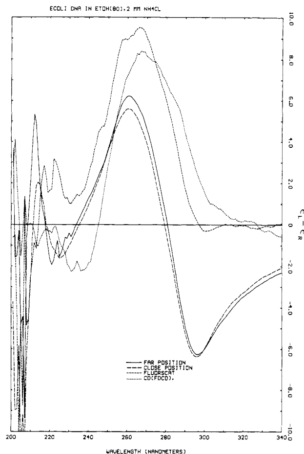
FIGURE 3: CD spectra of E. coli DNA-EtOH condensed particle as a function of measuring geometry. These condensates have obvious scattering components in the long-wavelength regions. Even when corrected by FDCD methods, this condensed DNA shows a CD spectrum different from the conservative CD of DNA in the B or C geometries (see Figure 5, this paper).
