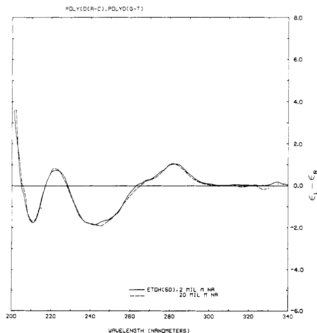
FIGURE 5: CD of poly[d(A-C)-d(G-T)] in 50% EtOH, 2 mM Na + , and 20 mM Na + . This is the so-called conservative CD of DNA reflecting a B or C secondary geometry.
