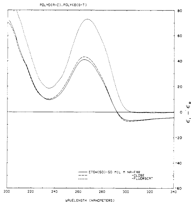
FIGURE 6: CD spectra of polymer in Figure 5 when the salt concentration is increased to 50 mM Na + . The signal increases by a factor of 40, and differential scattering components appear in the long-wavelength region.
