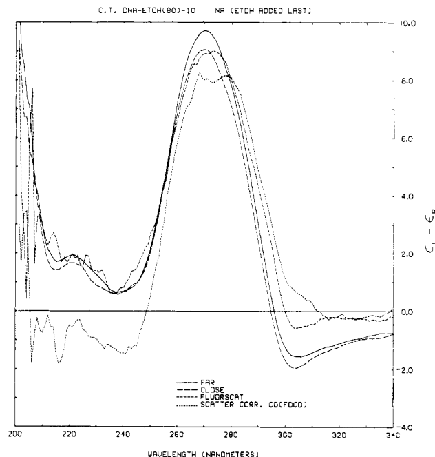
FIGURE 1: CD spectra of calf thymus DNA-EtOH condensate as measured by techniques having varying solid angles of light detection.
