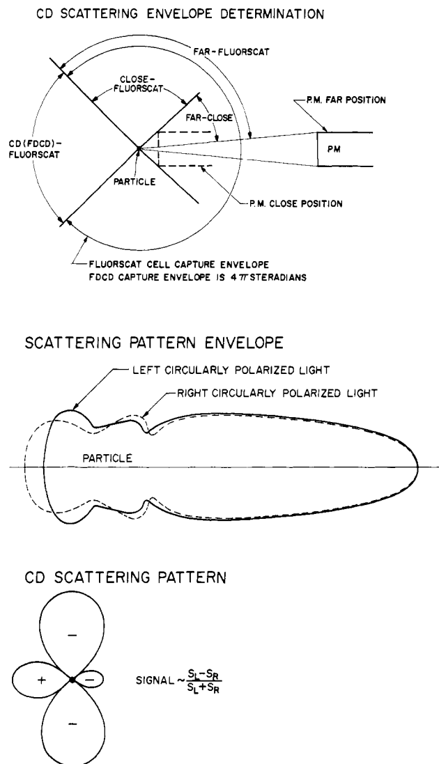
FIGURE 2: Diagrammatic representation of the CD scattering envelope of a hypothetical particle. Different sectors are measured by computing the proper differences between measuring methods. Thus, far minus close gives the forward scattering component, close minus fluorscat gives the side lobes, and fluorscat minus CD(FDCD) gives the backscattering component. CD(FDCD) means CD obtained from the FDCD measurement as described in the text.
